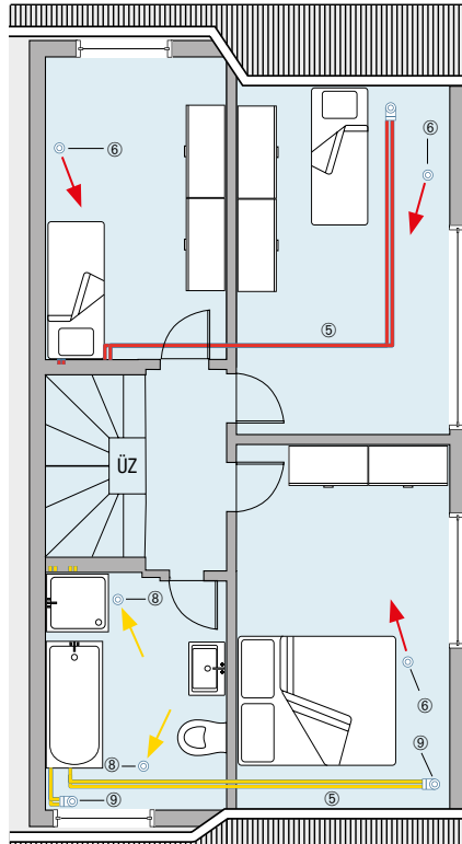
Obergeschoss (OG)
